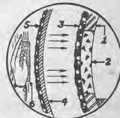
CROSS SECTION OF DAMAGED HULL
