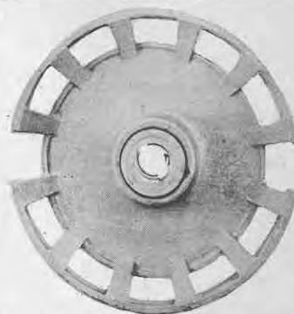
Test wheel replaces prop on the lower unit. (Photo and drawings courtesy Johnson Motors)
